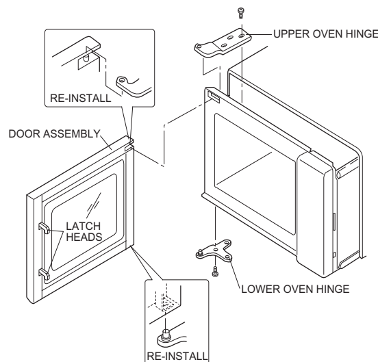
Figure C-5. Door Replacement and adjustment
