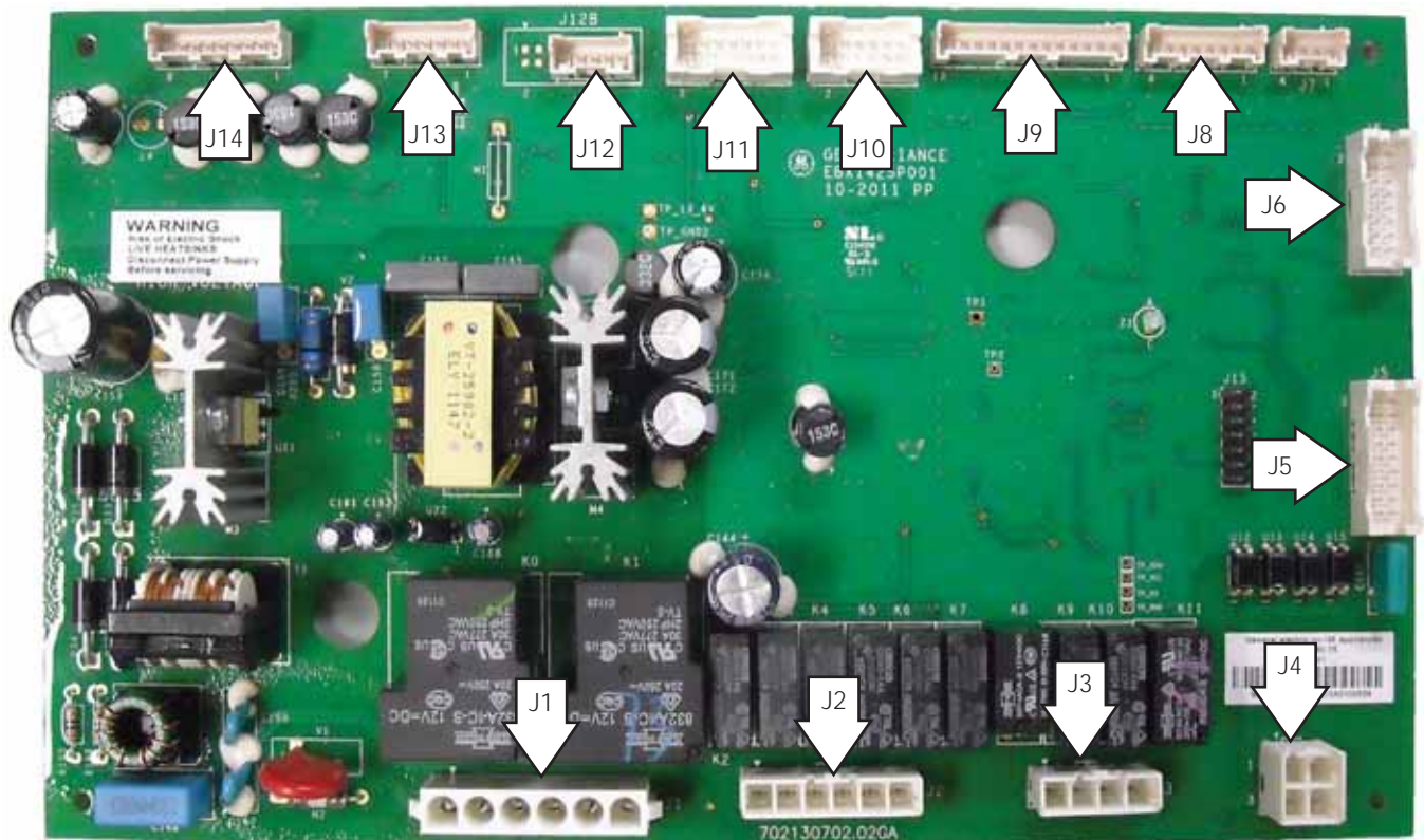
Main Control Board
