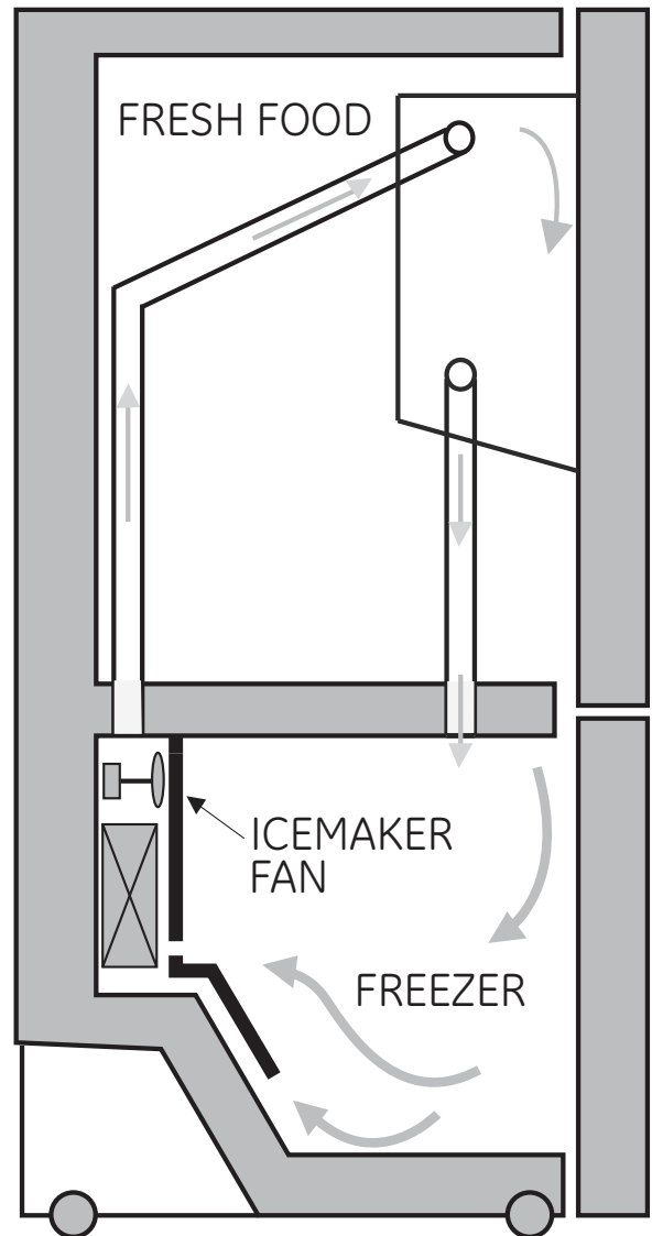
Ice System Air Flow (side view)
